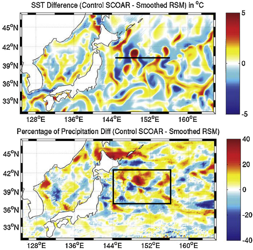
Fig. 10. Difference in SST [ ^{\circ} C] distribution (top) of Control SCOAR – Smoothed RSM for January 2001. Corresponding distribution of percentage difference in precipitation [mm/day] (bottom). Location of 40.5^{\circ} transect and intensified mesoscale region [boxed domain; 144\text{--}156^{\circ} E, 37\text{--}42^{\circ} N] marked on top and bottom figures respectively.
